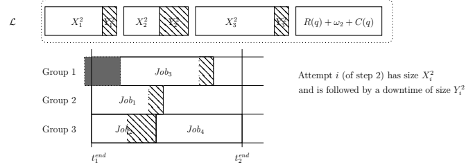
Figure 2: Zoom on macro-step 2 of the execution depicted in Figure 1, using the (X, Y) notation of Algorithm 2. Recall that Job_i has size X_i^j + Y_i^j for 1 \leq i \leq 3 , and Job_4 has size R(q) + \omega_2 + C(q) .
