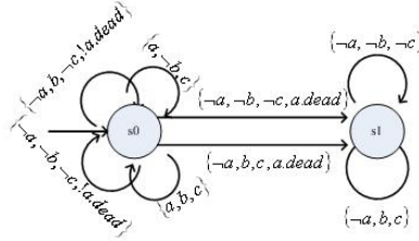
Figure 21: CTS of c = a \text{ concat } b
