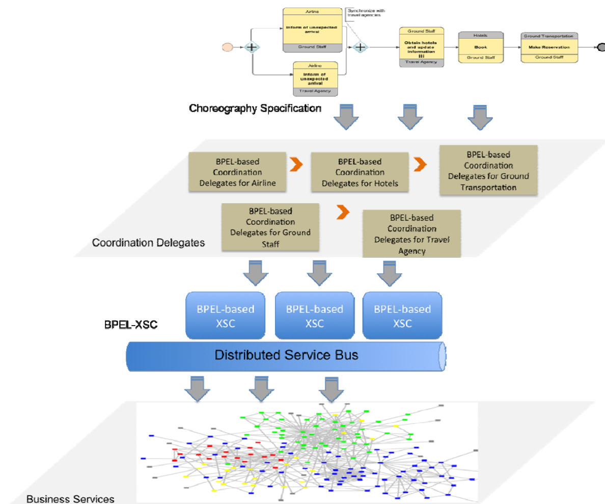
Figure 5-3. BPEL-based mapping of choreographies.
