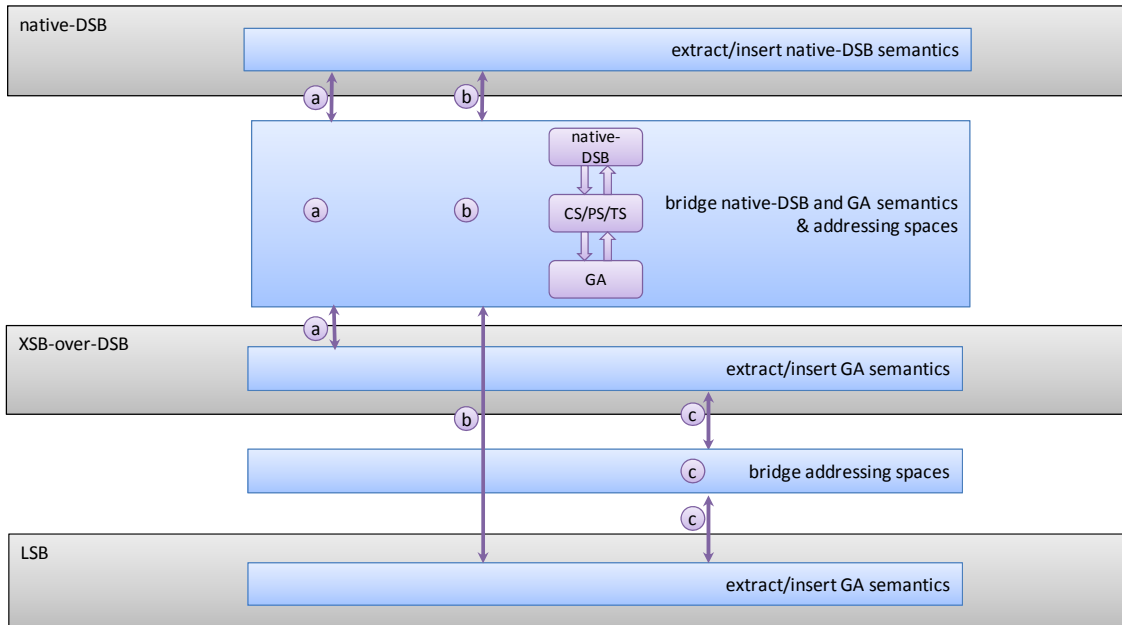
Figure 4-9. DSB-LSB Bridging.
