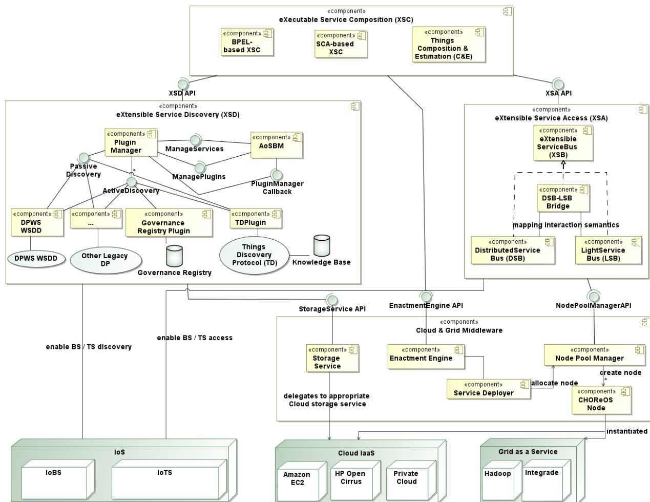
Figure 2-1. CHOReOS Middleware Architecture.
