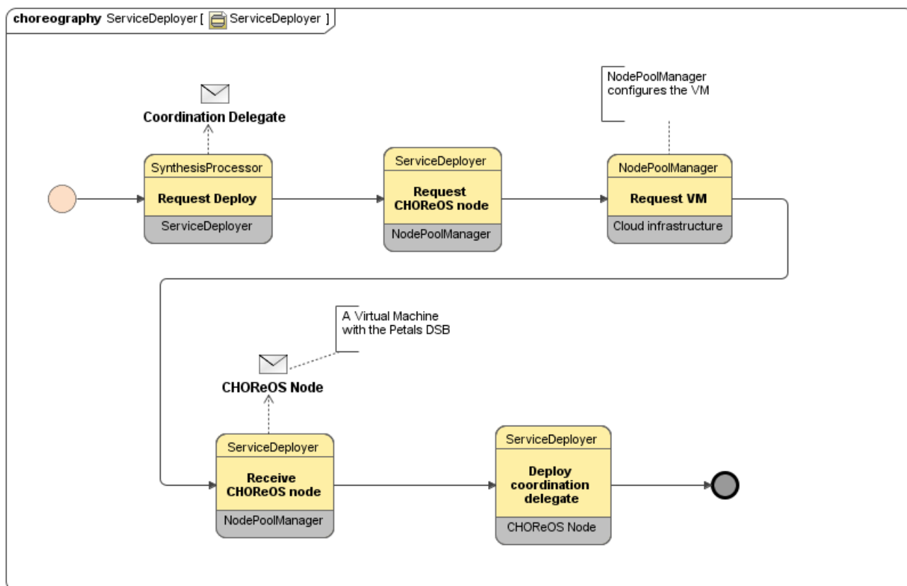
Figure 2.8: Coordination delegate deployment process
