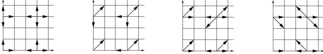
Fig. 1.1: Four famous examples, known as the simple, Kreweras', Gessel's and Gouyou-Beauchamps' walks, respectively
