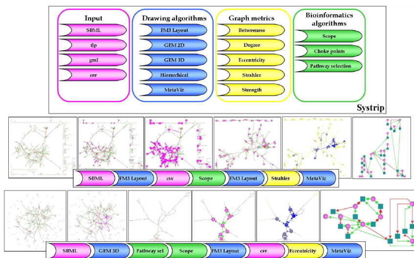
Figure 10: The Systrip pipeline was created to help biologists understand the metabolism of the tsetse fly parasite that causes sleeping sickness. First, through the generic perspective of Tulip and then through a custom Systrip perspective, we began to understand the task requirements, providing a visualization pipeline customized to the task of the biologist.
