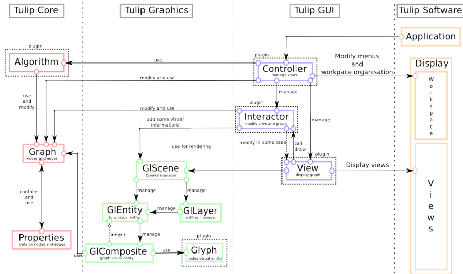
Figure 1: Tulip architecture overview. The Tulip framework consists of four packages. Tulip core provides an efficient data structures for relational data. Tulip graphics is a complete OpenGL rendering engine. Tulip-GUI is a collection of widgets built on top of Qt-Nokia library for the purpose of information visualization. Finally, Tulip software is an application for embedding algorithms, visualization techniques/interaction, and complete information visualization systems. All these packages can be dynamically extended through the plug-in architecture of Tulip.
