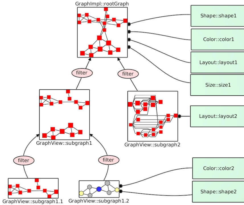
Figure 3: Graph Hierarchy: Tulip provides management of a hierarchy of subgraphs through an efficient filtering mechanism of graphs. For example, a graph with 1,000,000 nodes and 5,000,000 edges and 200,000 subgraphs requires 825 Mb on a 64-bit architecture. Furthermore, through an inheritance mechanism of properties of graph through that hierarchy, it maximizes the number of properties shared between subgraphs. For instance, the subgraph1.2 inherits the layout of the root graph. The inheritance mechanism is also able to redefine properties in subgraphs like one would do in an object oriented programming language. The subgraph2, for example, has redefined its layout but inherits the colors/sizes and shapes of its parent.
