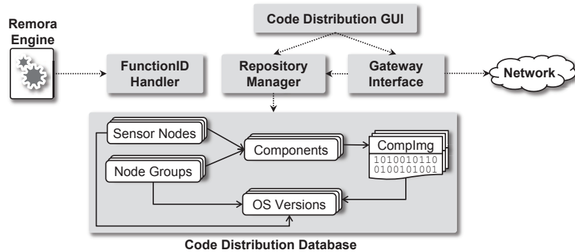
Fig. 10. The overall architecture of code repository and distribution server.
