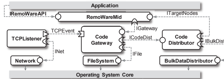
Fig. 11. REMOWARE configuration within the code propagator.
