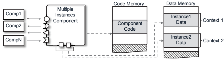
Fig. 6. A close-up of a multiple-instances REMORA component.
