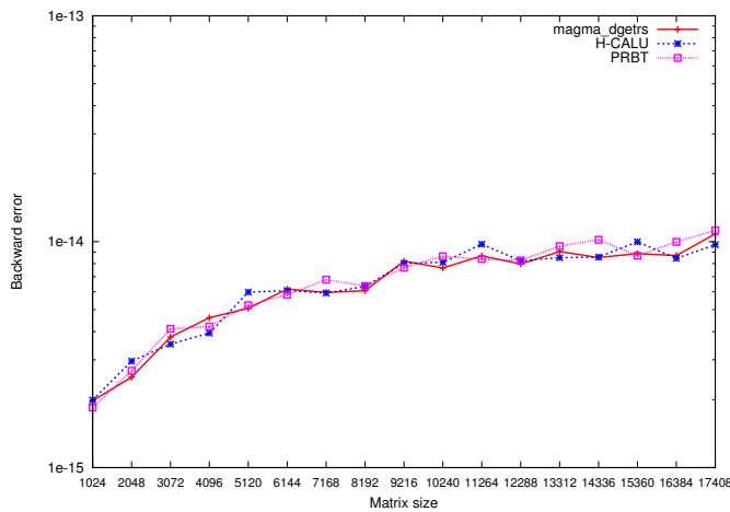
Figure 7: Comparison of componentwise backward error
