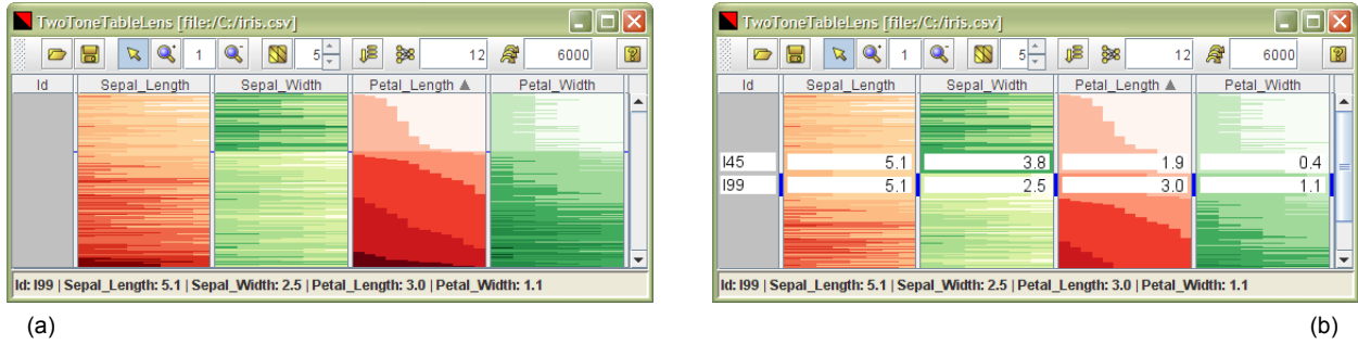
Figure 5. Iris dataset – (a) Data sorted with respect to petal length; (b) Rows adjacent to discontinuity are expanded to get detail information.
