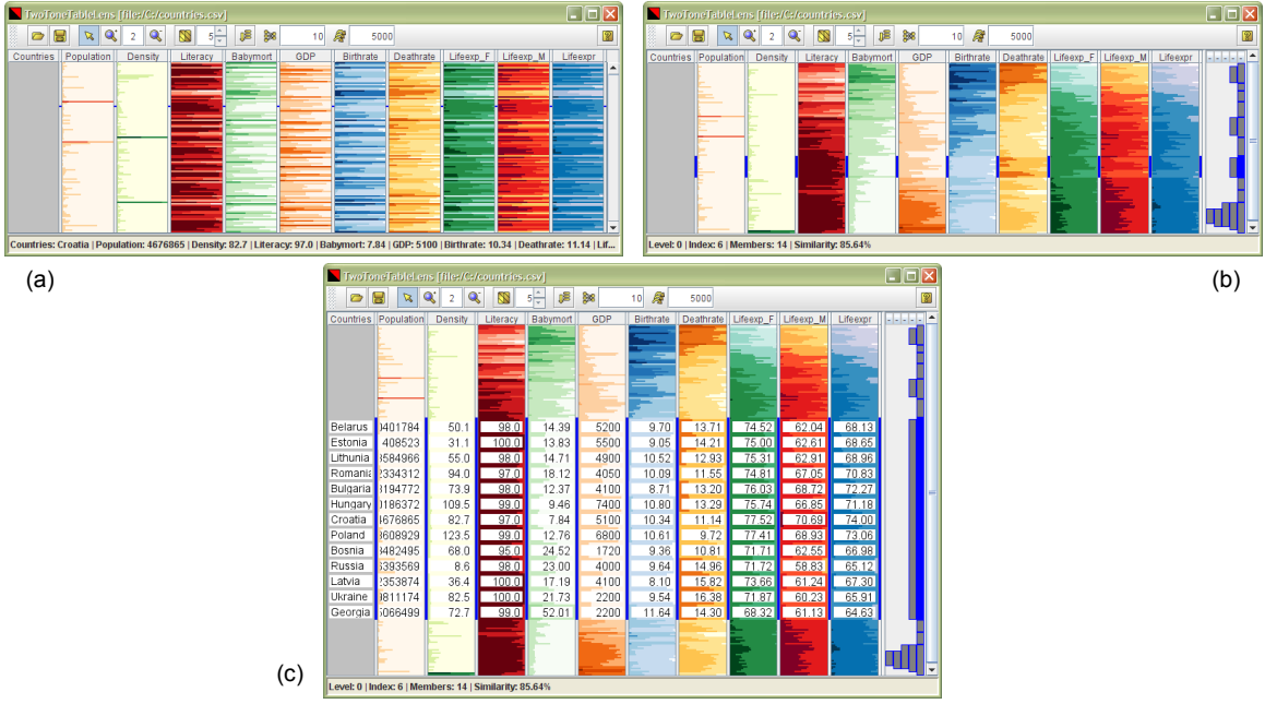
Figure 6. Countries dataset – (a) Unsorted view; (b) After clustering has been applied, a cluster of interest can be selected (denoted by blue bar); (c) Expanding that cluster reveals former east block countries.
