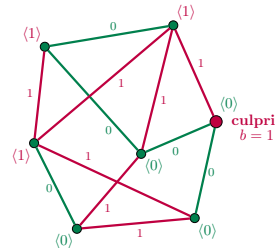
Fig. 1. Example of a dc-net.
