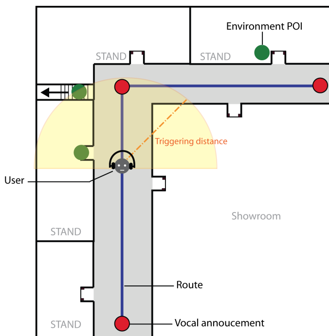
Figure 5: Radar Mode.
