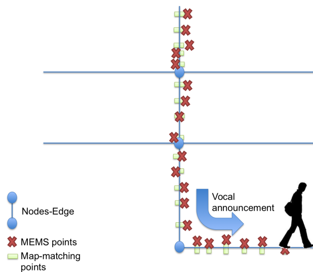
Figure 4: Map-matching.
