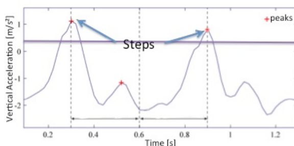
Figure 3: Step detection.
