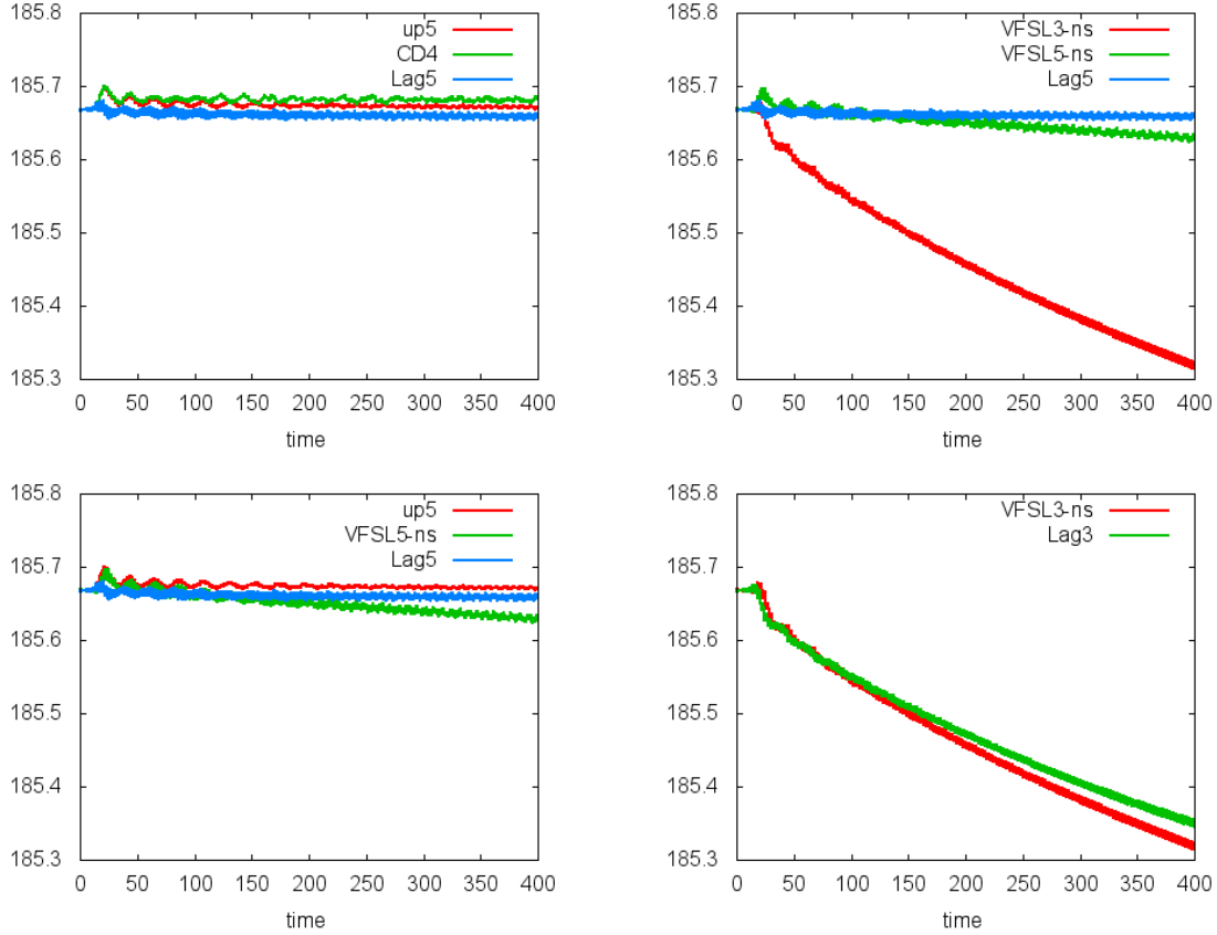
FIGURE 5. Bump on tail test: time evolution of the total energy for "Banks" methods (CD4 and up5), for the unsplit Vfs methods (Vfs3-ns and Vfs5-ns) and for semi-Lagrangian method (Lag3 and Lag5). N_x = N_v = 128 , \Delta t = 0.01 .
