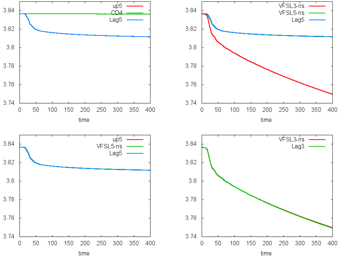
FIGURE 6. Bump on tail test: time evolution of the L^2 norm for "Banks" methods (CD4 and up5), for the unsplit Vfl methods (Vfl3-ns and Vfl5-ns) and for semi-Lagrangian method (Lag3 and Lag5). N_x = N_v = 128 , \Delta t = 0.01 .
