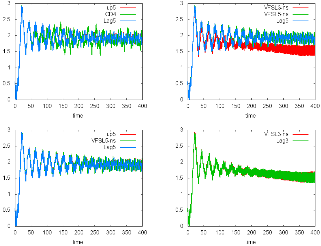
FIGURE 3. Bump on tail test: time evolution of the electric energy for "Banks" methods (CD4 and up5), for the unsplit Vfs methods (Vfs3-ns and Vfs5-ns) and for semi-Lagrangian method (Lag5). N_x = N_v = 128 , \Delta t = 0.01 .
