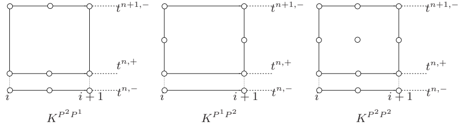
Figure 1: Examples of P^n P^m elements
