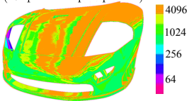
(c) Estimated variance (Required # light samples)
