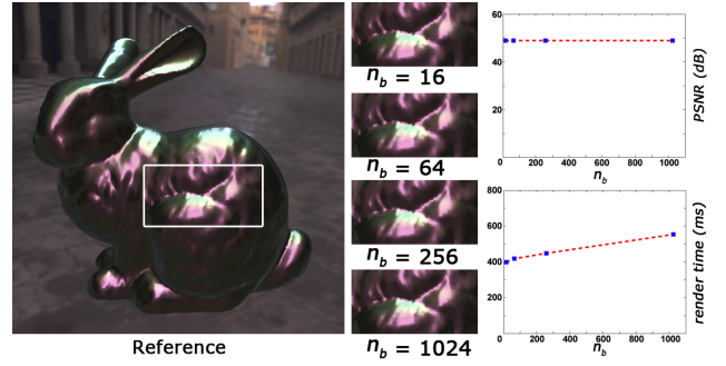
Figure 13: Effect of the number of sampled directions n_b for bandwidth computation on time (ms) and quality (PSNR). The data points in the plots are at n_b = 16, 64, 256, 1024 . The enlarged insets are virtually indistinguishable for the different n_b . The plots depict that fast bandwidth computation ( n_b = 16 ) is sufficient. Resolution: 512 \times 512 . Material: color-changing-paint3.
