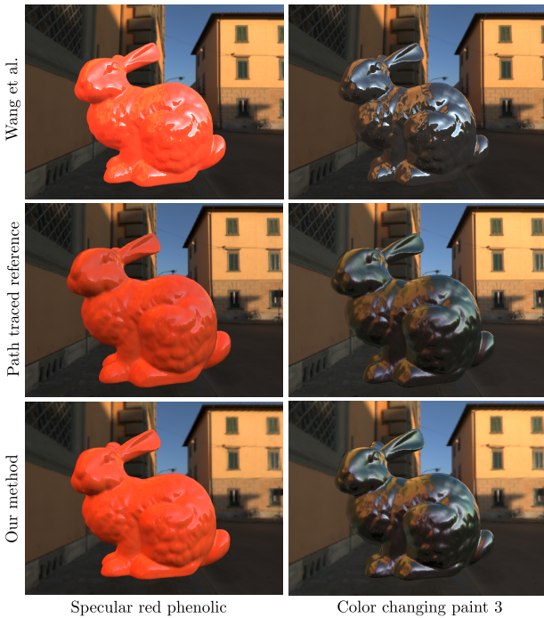
Figure 15: Comparison with related work [Wang et al. 2009]. Our algorithm results in pictures that are identical to ground truth, while [Wang et al. 2009] result in clear differences.
