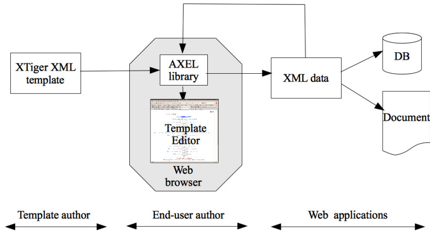
Figure 1: Architecture of XTiger+AXEL on-line document tool
