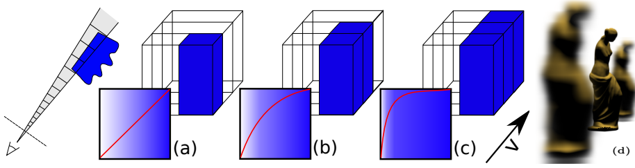
Figure 4: (a): A pixel is only half covered by opaque geometry, thus the fragment has an opacity \alpha = 0.5 . (b,c): Successively accumulating opacity by naive blending progressively saturates the final result, while it should stick to 0.5. This tends to thicken silhouettes of antialiased or unfocused shapes (d). I.e., the \alpha -blending model is wrong when fragments (or successive cone elements) are highly correlated, which is the case at silhouettes.
