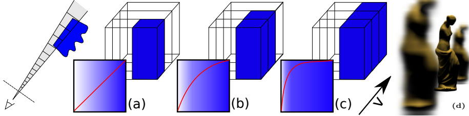
Figure 4: (a): A pixel is only half covered by opaque geometry, thus the fragment has an opacity \alpha = 0.5 . (b,c): Successively accumulating opacity by naive blending progressively saturates the final result, while it should stick to 0.5. This tends to thicken silhouettes of antialiased or unfocused shapes (d). I.e. , the \alpha -blending model is wrong when fragments (or successive cone elements) are highly correlated, which is the case at silhouettes.
