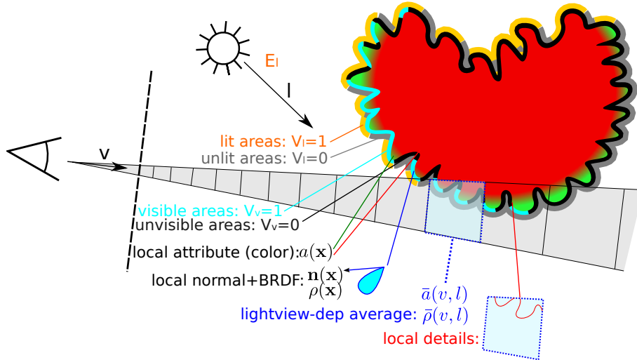
Figure 2: Context : rendering objects with complex subpixel details possibly correlated with depth within the coarse surface. The prefiltering must account that their contribution is correlated to their visibility from eye or light.
