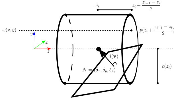
Figure 12: The bit corresponding to \omega(x, y) is set to 0 if one of the points p(z_i \pm \frac{z_{i+1} - z_i}{2}) is below the oriented cutting plane.
