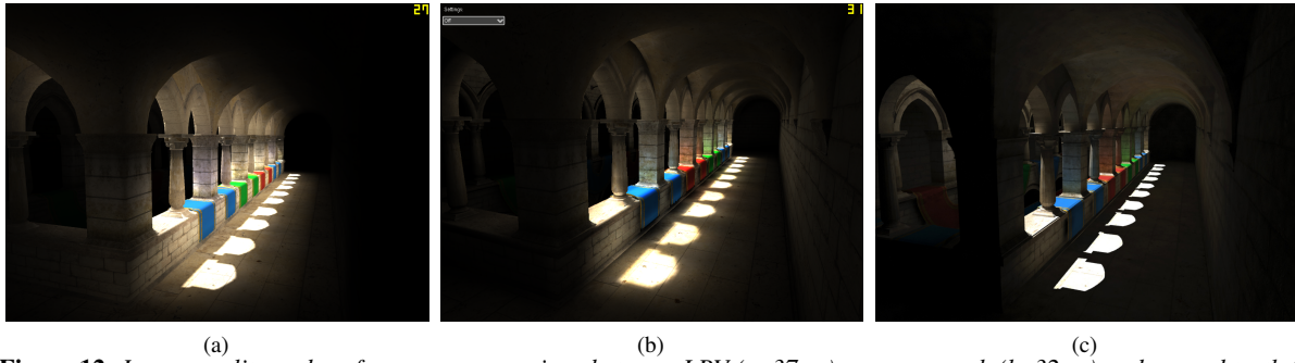
Figure 12: Image quality and performance comparison between LPV (a, 37ms), our approach (b, 32ms) and ground truth (c, 14"12s) rendered with Mental Ray.
