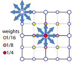
Figure 4: Lower-level voxels surround higher-level voxels. During MIP-mapping, shared voxels are “evenly distributed” resulting in gaussian weights.
