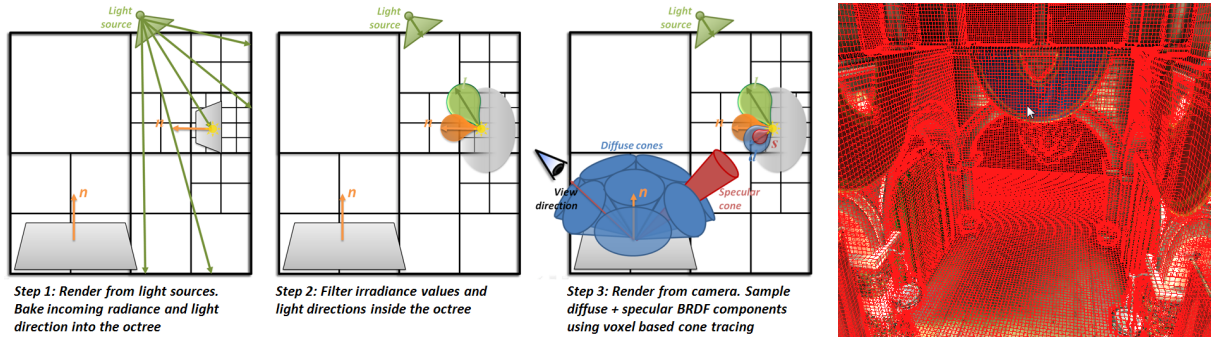
Figure 3: Left: Illustration of the three steps of our real-time indirect lighting algorithm. Right: Display of the sparse voxel octree structure storing geometry and direct lighting information.
