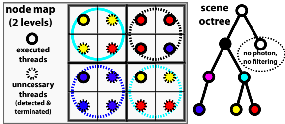
Figure 10: The node map (left) is constructed from the light-view map. It is hierarchical (like a MIP-map) and has several levels (large circles represent the next level). On the lowest level, a pixel contains the index of the node in which the corresponding photon is located. Higher levels contain the common lowest ancestor of all underlying nodes. This structure allows to reduce the number of threads launched during the filtering of the photons (dashed are stopped).
