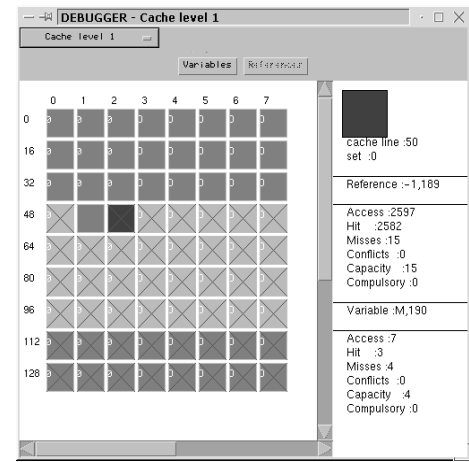
Figure 2: Debugger
