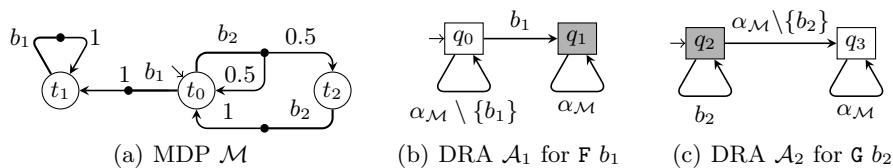
Fig. 14. The MDP and deterministic Rabin automata for Example 17
