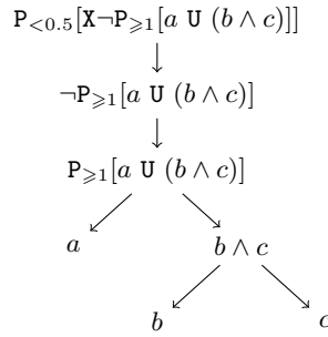
Fig. 7. The parse tree for a formula P_{<0.5}[X\neg P_{\geq 1}[a U (b \wedge c)]]
