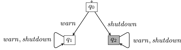
Fig. 8. DFA \mathcal{A}_A^{err} for the regular safety property \Phi_A in Example 12
