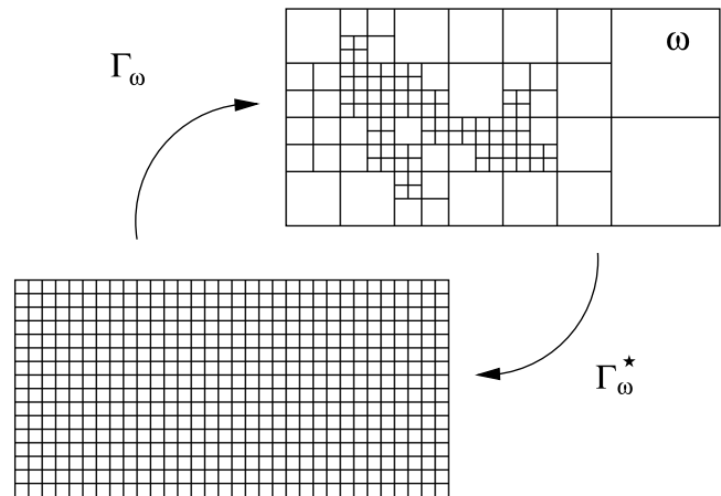
Figure 2. Schematic of the restriction operator \Gamma_\omega and of the prolongation operator \Gamma_\omega^* , which relate sources at finest scale with those on a multiscale representation \omega .
