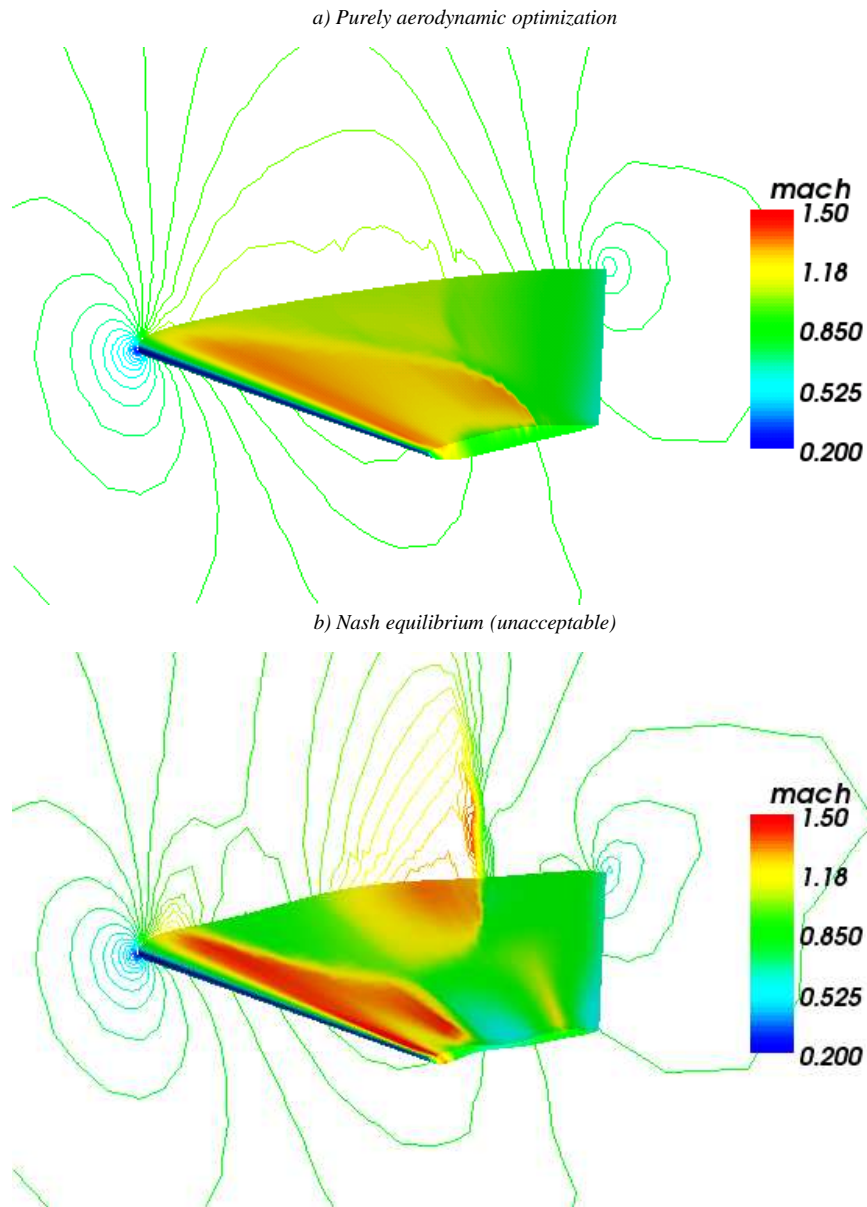
Fig. 9 Aero-structural shape optimization of a business jet wing; first split of territory, according to the primitive variables : shape and Mach number field : a) purely aerodynamic optimization, and b) Nash equilibrium.
