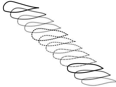
Fig. 2 An illustration of the NSGA in which an airfoil shape is optimized to reduce drag and maximize lift concurrently; in c) the upper-left airfoil has the highest lift, and the lower-right the lowest drag.
