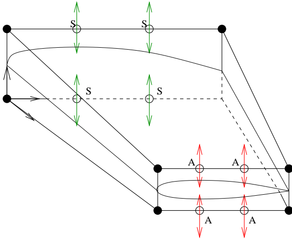
Fig. 10 Aero-structural shape optimization of a business jet wing; second split of territory, according to the primitive variables : parameters marked A are associated to aerodynamics, and those marked S to structural design.
