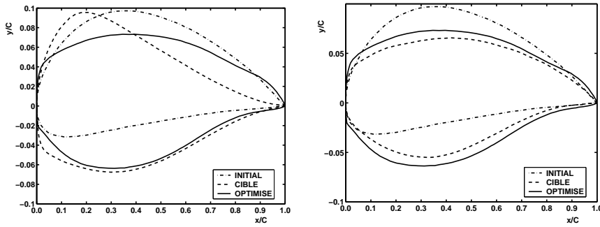
Fig. 5 Comparison between the optimized airfoil (solid line) with the initial airfoil and the target airfoil associated with the subsonic conditions of the first point (left), and the target airfoil associated with the transonic conditions of the second point (right); from [28]
