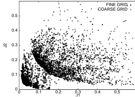
b) Discrete fronts of Pareto-optimal solutions (coarse and fine grids)
