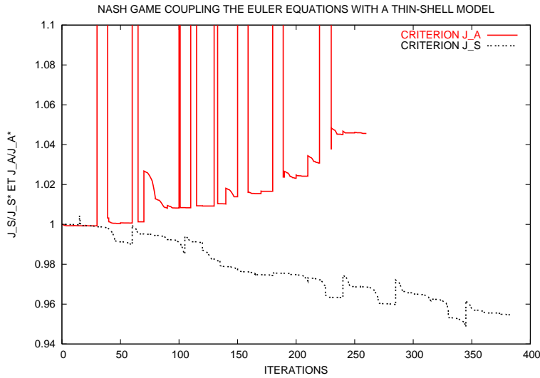
Fig. 11 Aero-structural shape optimization of a business jet wing; second split of territory, according to the primitive variables : convergence history of the two criteria
