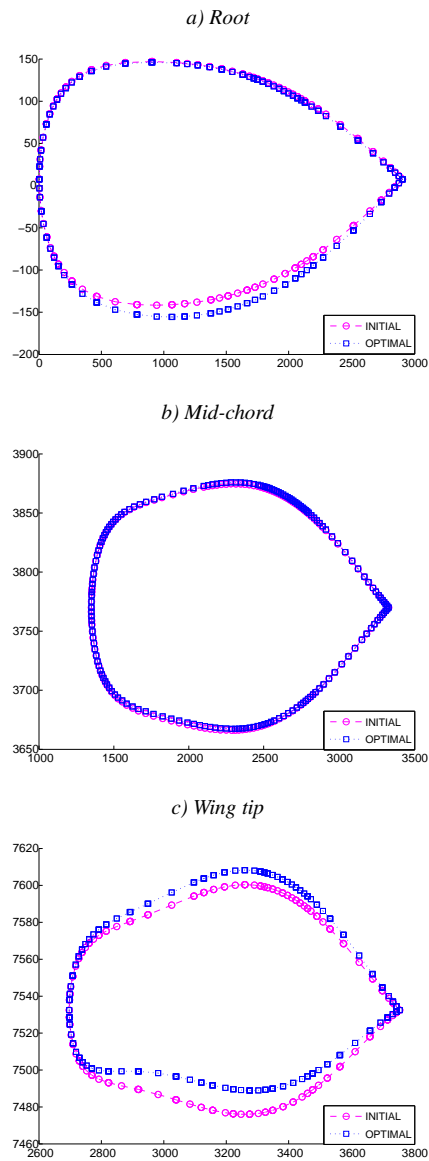
Fig. 14 Aero-structural shape optimization of a business jet wing; split of variables according to the orthogonal decomposition; cross-section variations at a) root, b) mid-chord, and c) wing tip.
