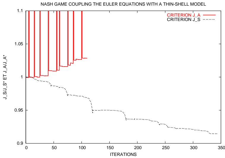
Fig. 13 Aero-structural shape optimization of a business jet wing; split of variables according to the orthogonal decomposition; convergence history of the two criteria (after 50 couplings).
