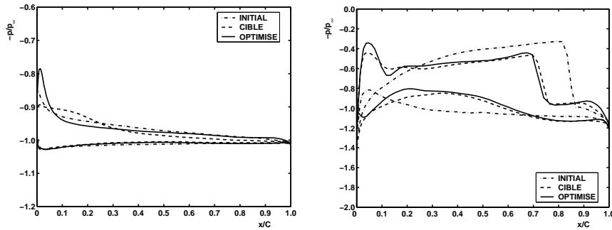
Fig. 6 Pressure distributions over the initial, target and optimized (solid line) shapes in the subsonic conditions of the first point (left), and in the transonic conditions of the second point (right); from [28]
