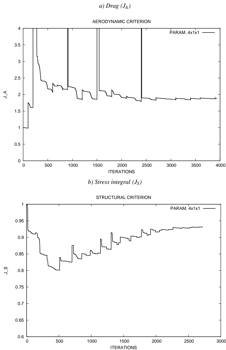
Fig. 8 Aero-structural shape optimization of a business jet wing; first split of territory, according to the primitive variables : convergence history of the aerodynamic and structural criteria.
