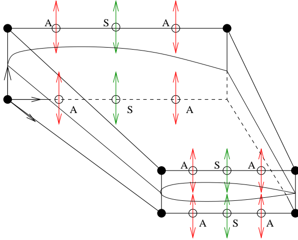
Fig. 7 Aero-structural shape optimization of a business jet wing: first split of territory, according to the primitive variables : parameters marked A are associated to aerodynamics, and those marked S to structural design.
