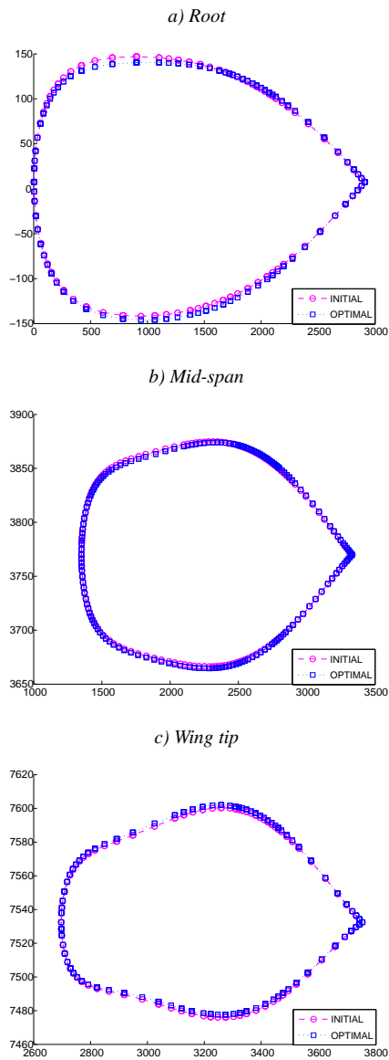
Fig. 12 Aero-structural shape optimization of a business jet wing; second split of territory, according to the primitive variables : cross-section variations at a) root, b) mid-span, and c) wing tip.
