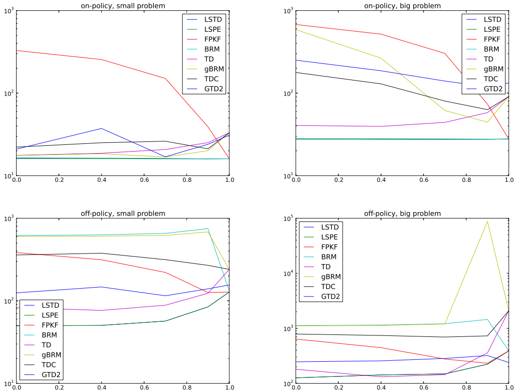
Figure 1: Sensitivity of performance of the algorithms ( y -axis, in logarithmic scale) with respect to the eligibility trace parameter \lambda ( x -axis). Left: Small problem ( \mathcal{G}(30, 4, 2, 8) ), right: Big problem ( \mathcal{G}(100, 10, 3, 20) ). Top: on-policy learning ( \pi = \pi_0 ), bottom: off-policy learning ( \pi \neq \pi_0 ).
