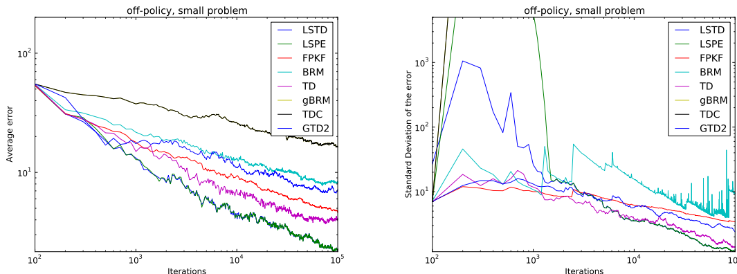
Figure 4: Performance for small problems ( \mathcal{G}(30, 4, 2, 8) ), off-policy learning ( \pi \neq \pi_0 ) (left: average error, right: standard deviation).
