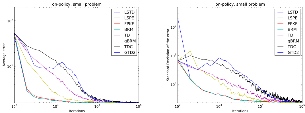
Figure 2: Performance for small problems ( \mathcal{G}(30, 4, 2, 8) ), on-policy learning ( \pi = \pi_0 ) (left: average error, right: standard deviation).
