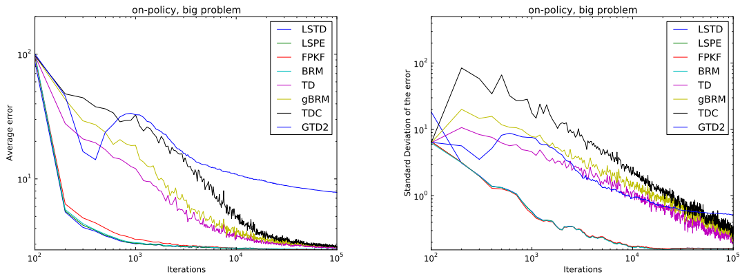
Figure 3: Performance for big problems ( \mathcal{G}(100, 10, 3, 20) ), on-policy learning ( \pi = \pi_0 ) (left: average error, right: standard deviation).
