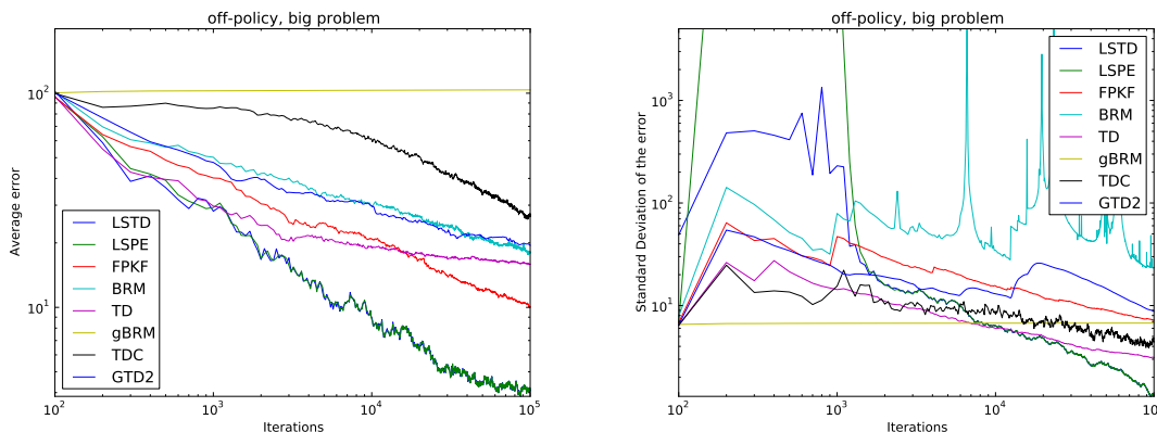
Figure 5: Performance for big problems ( \mathcal{G}(100, 10, 3, 20) ), on-policy learning ( \pi \neq \pi_0 ) (left: average error, right: standard deviation).
