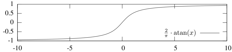
2: Limiting non-linear function
