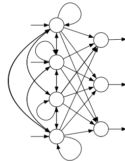
4: Iris network
