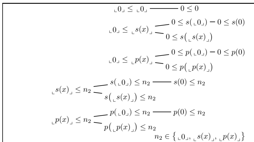
Figure 1: Sufficient completeness of \leq
