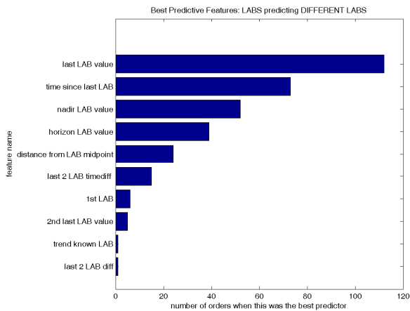
Figure 5. The most influential temporal feature categories for predicting lab order decisions with other lab features.
