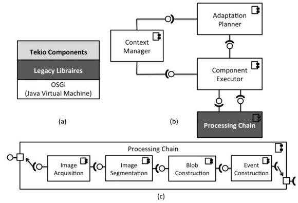
Figure 1: Tekio (a) Software Layers (b) Generic Architecture (b) Domain-specific Architecture
