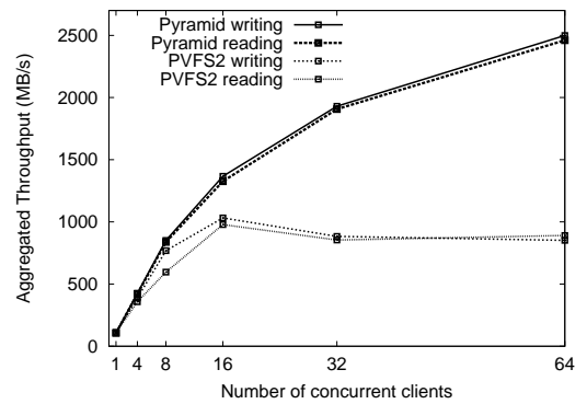
Figure 4: Strong scalability: fixed total domain size, increasing number of client processes
