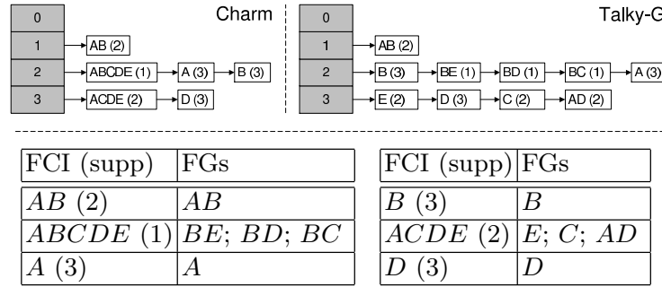
Fig. 4. Top: hash tables for dataset \mathcal{D} with min\_supp = 1 . Top left: hash table of Charm containing all FCIs. Top right: hash table of Talky-G containing all FGs. Bottom: output of Touch on dataset \mathcal{D} with min\_supp = 1
