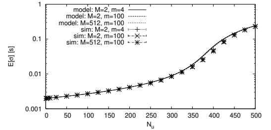
Figure 3: System cycle duration is affected by the number of users. It slightly grows with m and is almost insensitive to M .
