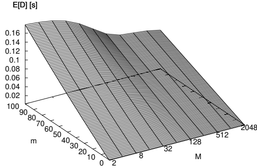
Figure 6: Access delay (independent on the number of users).
