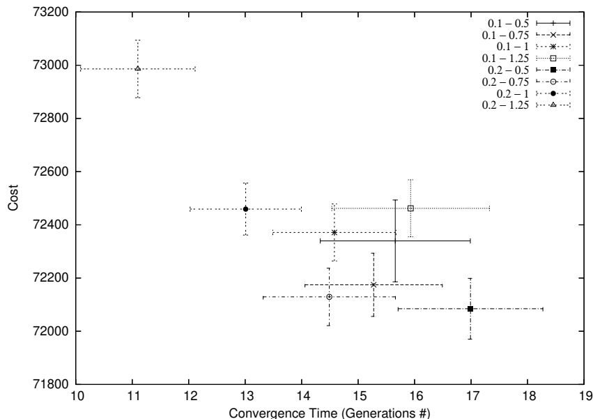
Figure 9: Cost function value vs. convergence time for various values of the noise parameters, 95% confidence interval.
