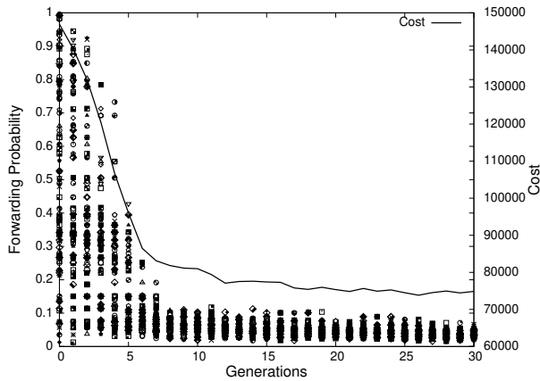
Figure 7: Cost function and forwarding evolution as a function of the generation number, N = 100 nodes.
