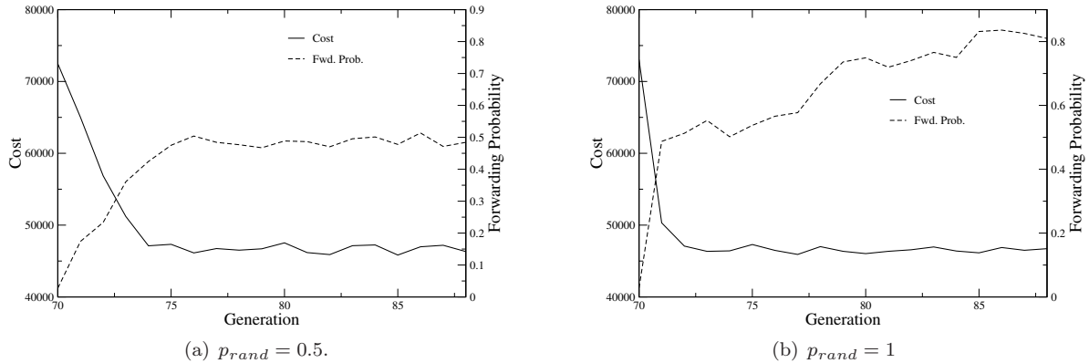
Figure 11: Performance of the modified scheme (in terms of cost function value and average forwarding probability) in a dynamic scenario, p_{rand} \in \{0, 5, 1\} , N dropping from 100 to 25.
