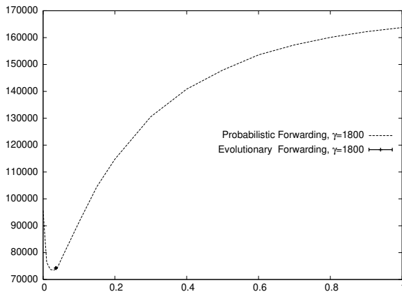
Figure 8: Cost function value as a function of the forwarding probability (statically set) and comparison with the results from the proposed evolutionary forwarding scheme.
