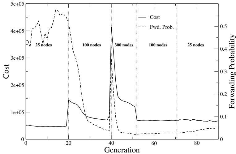
Figure 10: Dynamic scenario: cost function value and average forwarding probabilities versus generation number.
