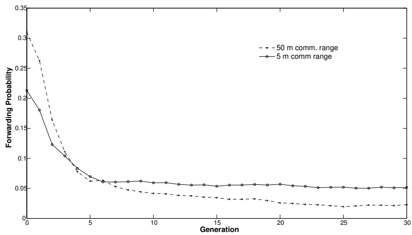
(a) Forwarding probability over generations.
