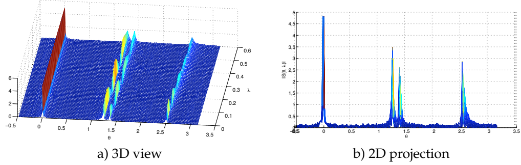
Figure 1: Spectrum of the linear chirp example
