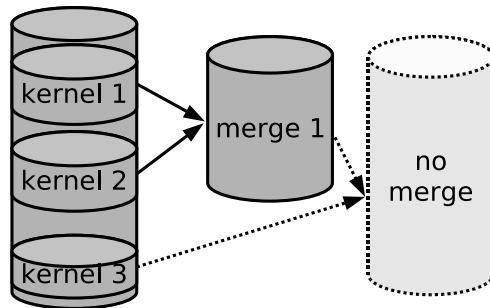
Fig. 6. Merging kernels
