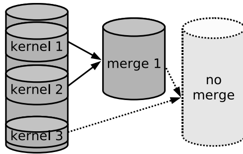
Fig. 6. Merging kernels
