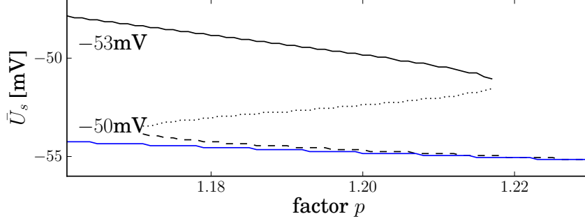
Figure 7: Stationary solutions in a network of excitatory and inhibitory neurons and synapses subjected to tonic inhibition. The given values -53\text{mV} and -50\text{mV} are the mean firing thresholds of excitatory neurons \Theta_e and reflect the absence (black lines) and presence (blue line) of tonic inhibition. For \Theta_e = -53\text{mV} , the top branch (solid line) and bottom branch (dashed line) are linearly stable (analysis not shown), whereas the centre branch (dotted line) is unstable. Other parameters are \sigma^2 = 1.0\text{mV}^2 , N_0 = 1 , \Delta = 1\text{ms} , \tau = 1.0\text{ms} , a_e = 40\text{mVs} , a_i = 80\text{mVs} , \Theta_i = -62\text{mV} . The stationary state is given by \bar{U}_s = \bar{V} + V_r , \bar{V} obeys Eq. (13) and V_r = -70\text{mV} is the neuron resting potential.
