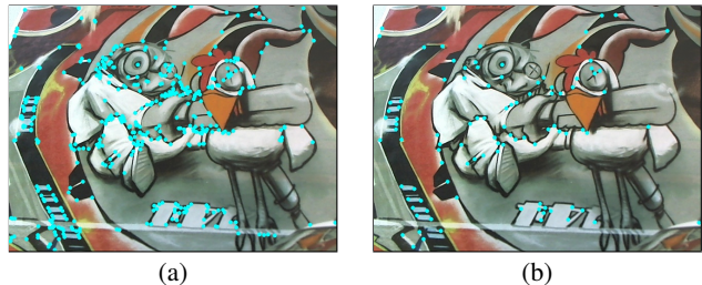
Figure 4: Keypoint selection. FAST was applied to Figure 3(a). (a) 427 keypoints were extracted in total. (b) 100 keypoints were extracted by setting the minimum distance as 10 pixels and the maximum number of keypoints as 100.
