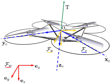
Fig. 7. Frame definitions.
