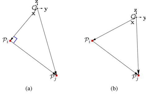
Fig. 2. Configuration of the two points in object frame \mathcal{F}_O = (\mathcal{O}, x, y, z) . (a) Specific case presented in [22] and (b) general case.
