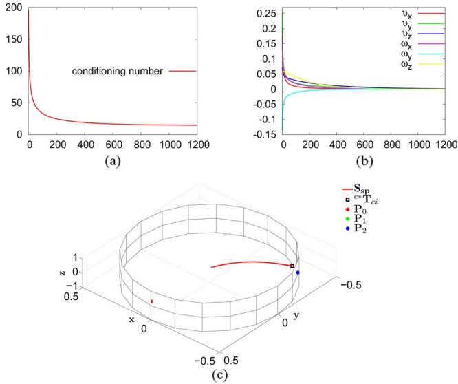
Fig. 10. Robustness w.r.t. modeling errors using the new set s_{sp} . (a) Conditioning number of the block matrix \mathbf{L}_v , (b) computed camera velocities (in meters per second and radians per second), and (c) camera Cartesian trajectories.
