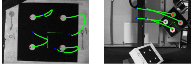
Fig. 4. Subsystem-based fusion \mathbf{C}_\# . Unweighted velocity contributions and trajectories for eye-in-hand (left) and eye-to-hand (right) cameras. The eye-to-hand contribution is more important, the eye-in-hand camera nearly loses some features
