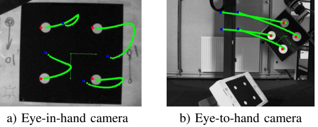
Fig. 4. Subsystem-based fusion \mathbf{C}_\# . Unweighted velocity contributions and trajectories for eye-in-hand (left) and eye-to-hand (right) cameras. The eye-to-hand contribution is more important, the eye-in-hand camera nearly loses some features
