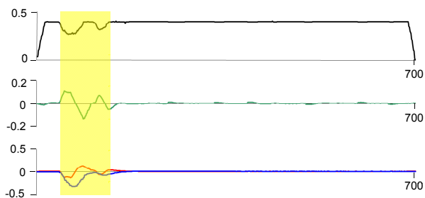
Fig. 6. Relevant variables in experiment 3: v (black, in \text{ms}^{-1} ), \omega (green, in \text{rad s}^{-1} ), \varphi (blue, in rad) and \dot{\varphi} (red, in \text{rad s}^{-1} ). The iterations with non-null H are highlighted in yellow.
