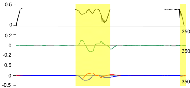
Fig. 5. Relevant variables in experiment 2: v (black, in \text{ms}^{-1} ), \omega (green, in \text{rad s}^{-1} ), \varphi (blue, in rad) and \dot{\varphi} (red, in \text{rad s}^{-1} ). The iterations with non-null H are highlighted in yellow.
