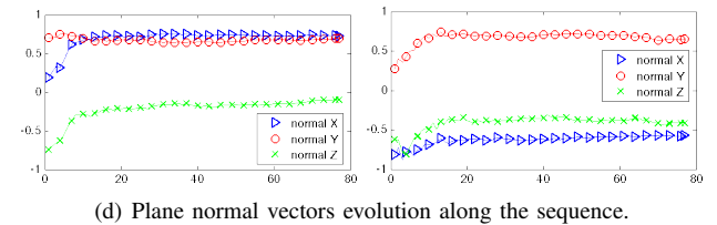
Fig. 5. Straight motion along 2.40 m. The final position error is 10 cm in 3D leading to an error ratio over the path length of around 4%. Note that the smallest plane in images (a) and (b) is not vertical, that is why its Z component is not 0.
