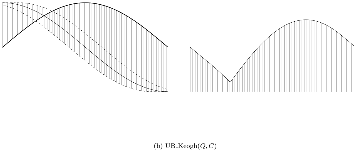
Figure 2: Example of \text{LB\_Keogh} and \text{UB\_Keogh} . U and L are defined as in [5]. The right hand side of each figure shows the overall area accounted for when computing each bound.
