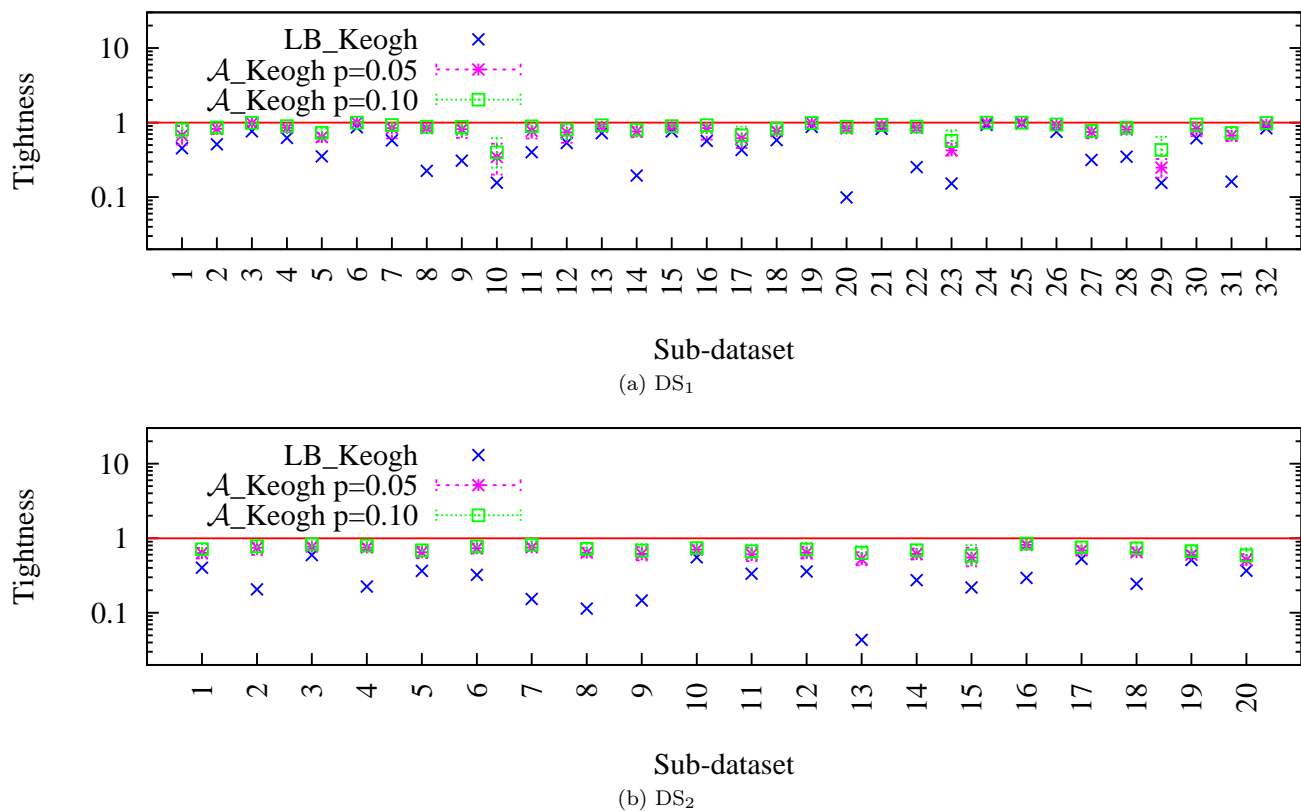
Figure 4: Median of tightness and its quartiles for \mathcal{A} .Keogh compared to the tightness of LB.Keogh.
