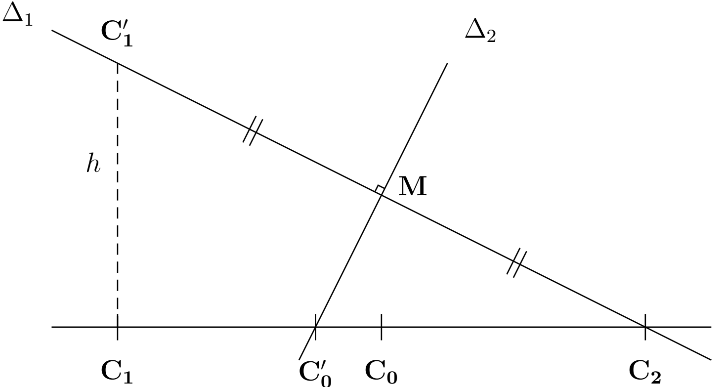
Figure 6: Balancing k -means for the k = 2 case.
