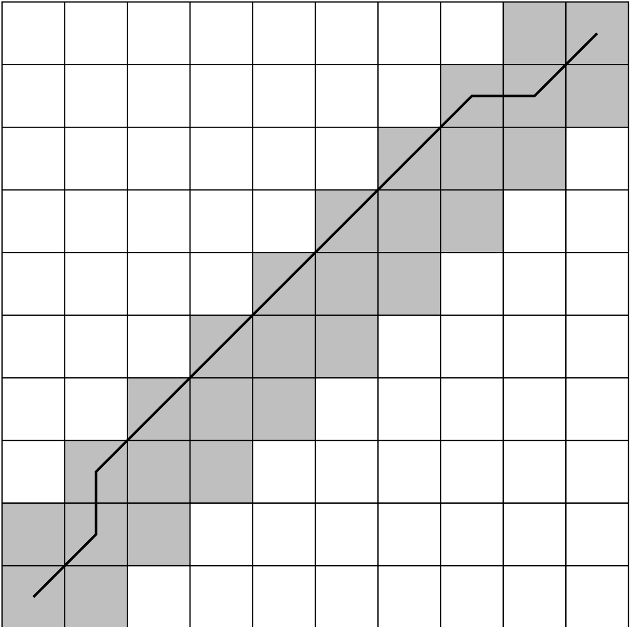
Figure 1: Example of a DTW path constrained by a Sakoe-Chiba band. Admissible paths are restricted to the gray area.
