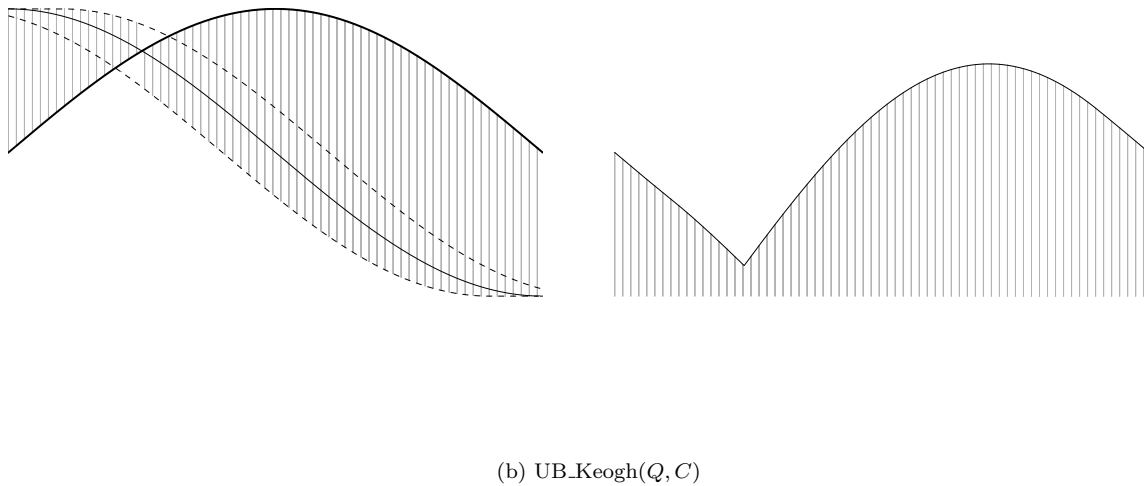
Figure 2: Example of LB\_Keogh and UB\_Keogh . U and L are defined as in [5]. The right hand side of each figure shows the overall area accounted for when computing each bound.
