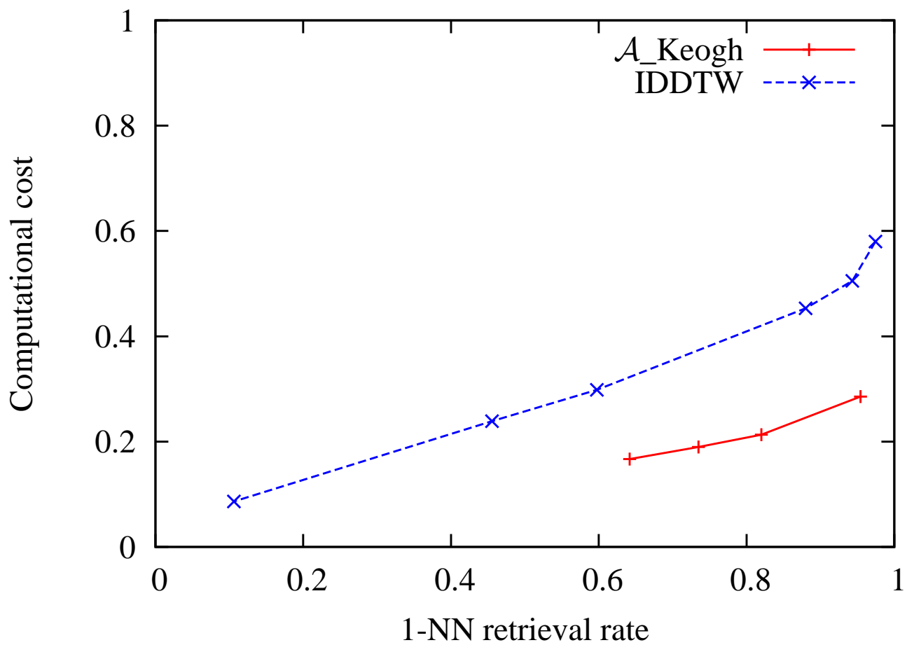
Figure 4: Comparison of IDDTW and \mathcal{A}_{Keogh} in terms of cost versus accuracy. The cost is defined as the number of elementary operations involved in the search process and accuracy is expressed in terms of 1-NN retrieval rate.
