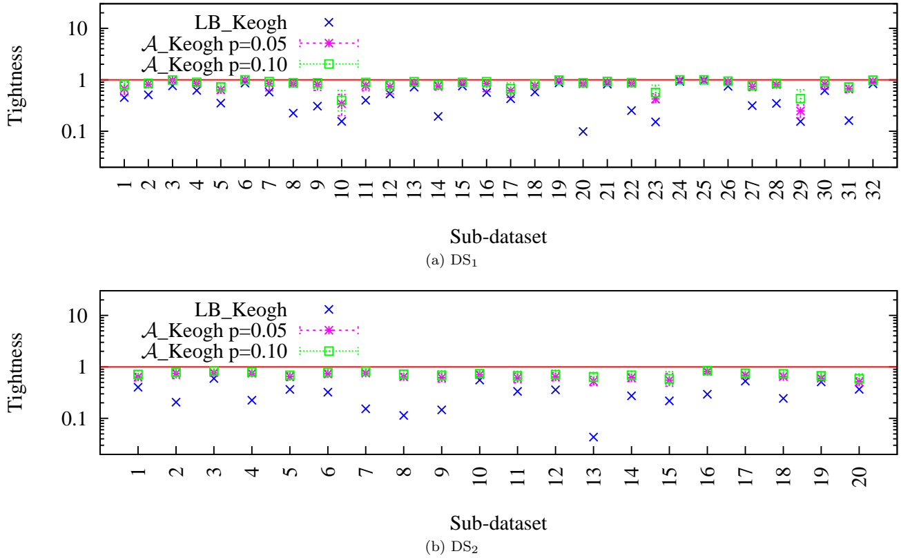
Figure 3: Median of tightness and its quartiles for \mathcal{A} .Keogh compared to the tightness of LB.Keogh.
