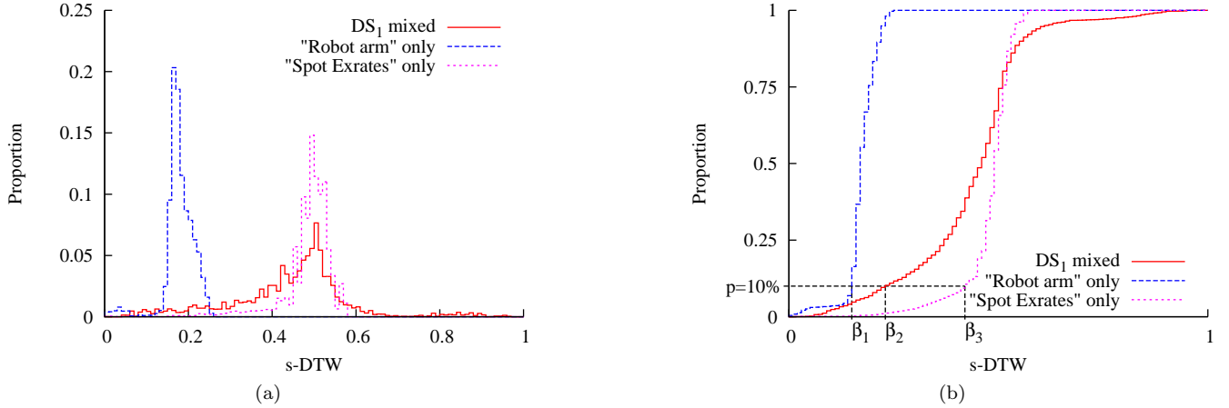
Figure 2: Experimental probability density function (a) and cumulative density function (b) for the whole merged dataset DS_1 and for its subdatasets “Robot Arm” (labeled #20 later) and “Spot Exrates” (labeled #24 later).
