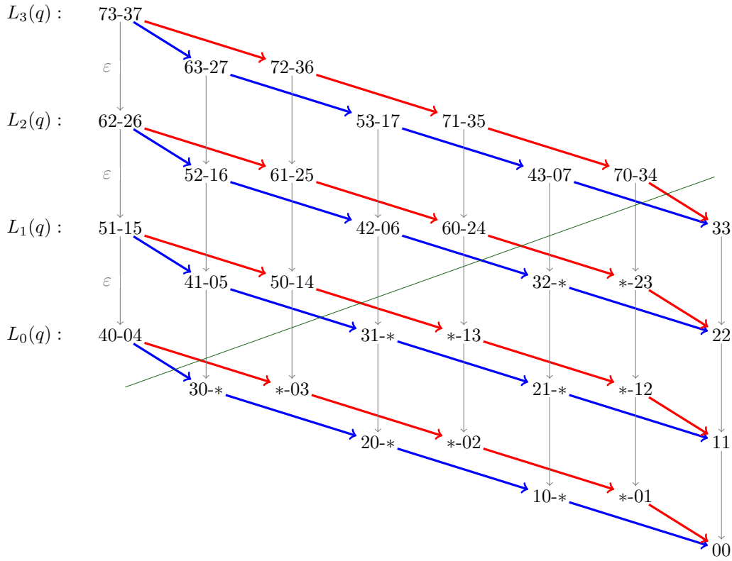
Fig. 1: Structure of q -Harmonic polynomials of G(4, 2) . For short, the q -harmonic binomial \langle d \rangle_4 x^\alpha y^\beta - \langle a \rangle_4 x^{\alpha'} y^{\beta'} is denoted “ \alpha\beta - \alpha'\beta' ”. Similarly, the q -harmonic monomial x^\alpha y^\beta is denoted “ \alpha\beta ”, “ \alpha\beta -*”, or “*- \alpha\beta ”. The blue (resp. red) arrows denote the action of the would be q -analogues of the operators \partial_x and \partial_y within each layer L_i . The gray arrows denote the action of the operator \varepsilon = e_2(\partial_X) = \partial_x \partial_y (recall that it changes the value of q ). The green line separates the q -harmonic monomials and binomials.
