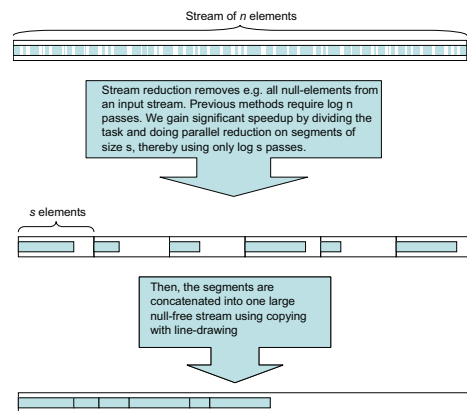
Figure 7: Our hierarchical stream reduction algorithm removes all null-elements from the input stream. We split the stream into small components of a fixed size, s , then run a standard parallel stream reduction on each component (in \log s passes). Finally, we concatenate the resulting segments in one render pass using line drawing.
