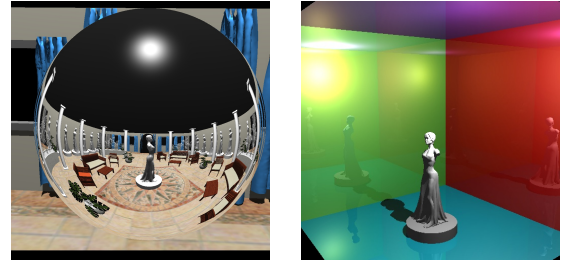
Figure 12: Our algorithm performs nicely even when the top levels have a large extent in the angular (a) or spatial (b) domain (512×512 pixels).
