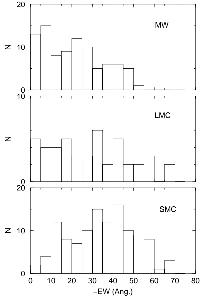
Fig. 2. Distributions of Be stars versus the EW of the H \alpha emission line. Top: in the MW from Dachs et al. (1992), Andriolat & Fehrenbach (1982) and Andriolat (1983); middle: in the LMC from Paper I; bottom: in the SMC (this study).
