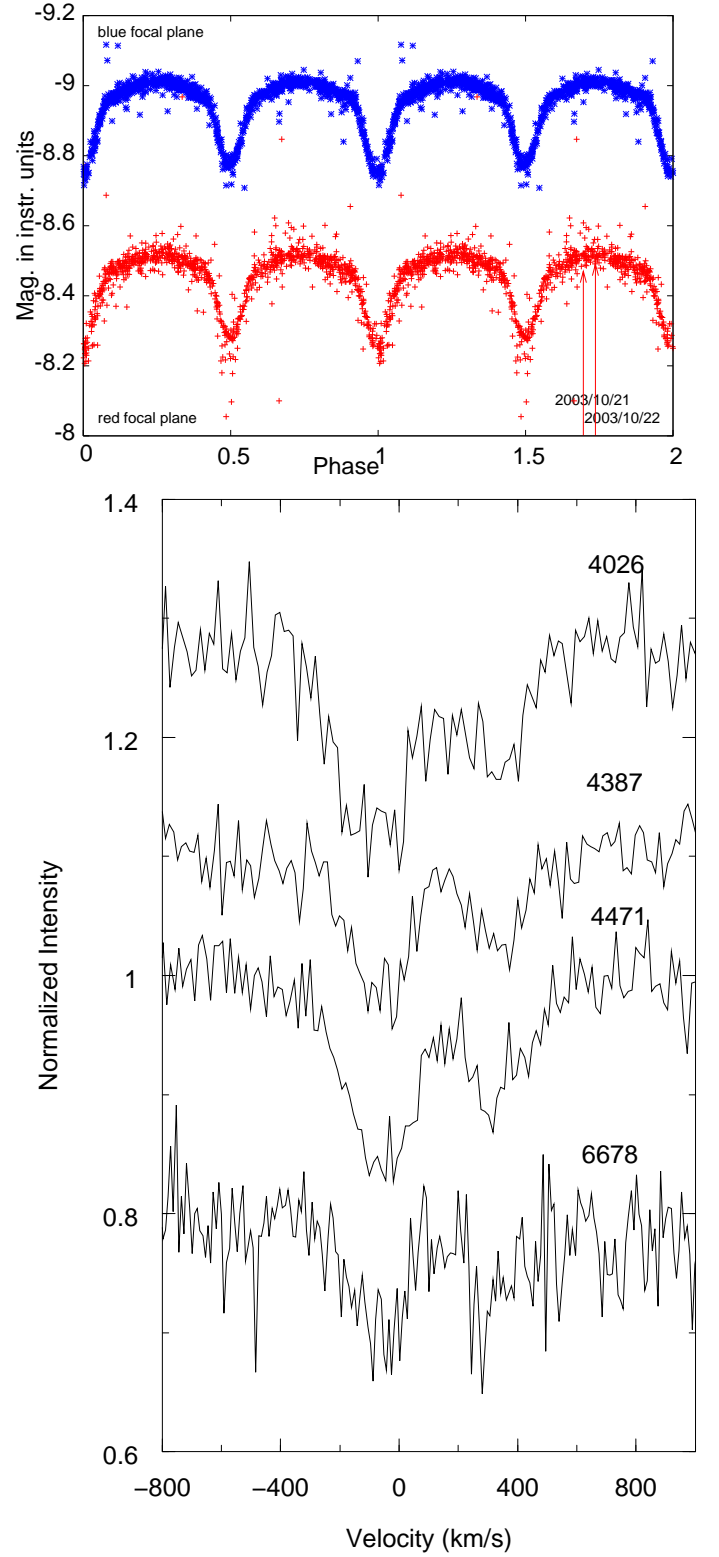
Fig. 10. SMC5_023641. Top: light curve folded in phase with P=2.010 d. Bottom: Helium lines taken at \phi=0.70 for the blue ones and at \phi=0.74 for the red one.
