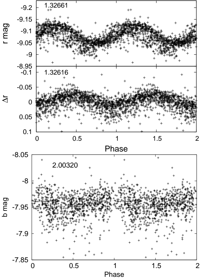
Fig. 13. Be SMC5_2232 folded in phase: top with f_1=1.32661\text{ c d}^{-1} , middle with f_2=1.32616\text{ c d}^{-1} after prewhitening for f_1 . Bottom: Be SMC5_3296 folded in phase with f=2.00320\text{ c d}^{-1}
