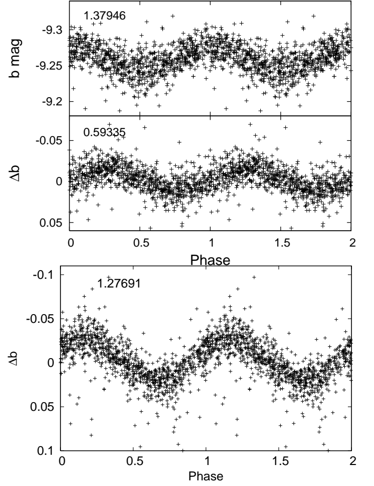
Fig. 14. Be SMC5_13978 folded in phase: top with f_1=1.37946\text{ c d}^{-1} , middle with f_2=0.59335\text{ c d}^{-1} after prewhitening for f_1 . Bottom: Be SMC5_14212 folded in phase with f=1.27691\text{ c d}^{-1} .
