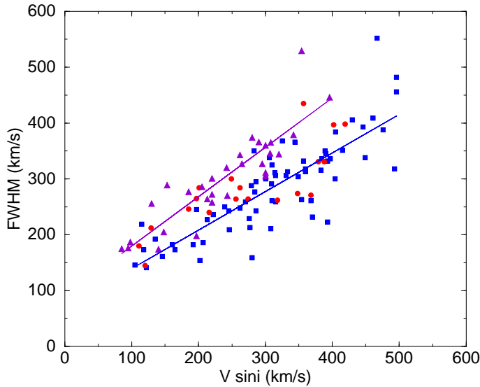
Fig. 3. FWHM of the H\alpha emission line as a function of V \sin i for Be stars with symmetric H\alpha profiles and EW\alpha > 20 Å. Squares correspond to Be stars in the SMC, circles to Be stars in the LMC from Paper I, and triangles to Be stars in the MW from Dachs et al. (1992), Andriolat & Fehrenbach (1982) and Andriolat (1983). The linear regression for samples in the SMC and MW is shown.
