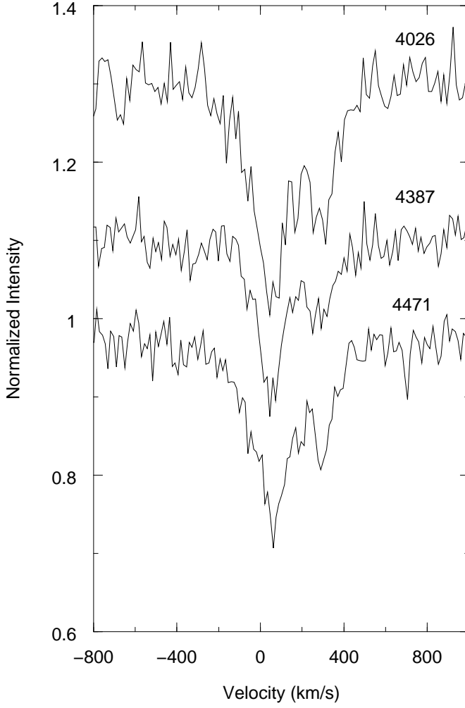
Fig. 11. Blue helium lines of SMC5_052663
